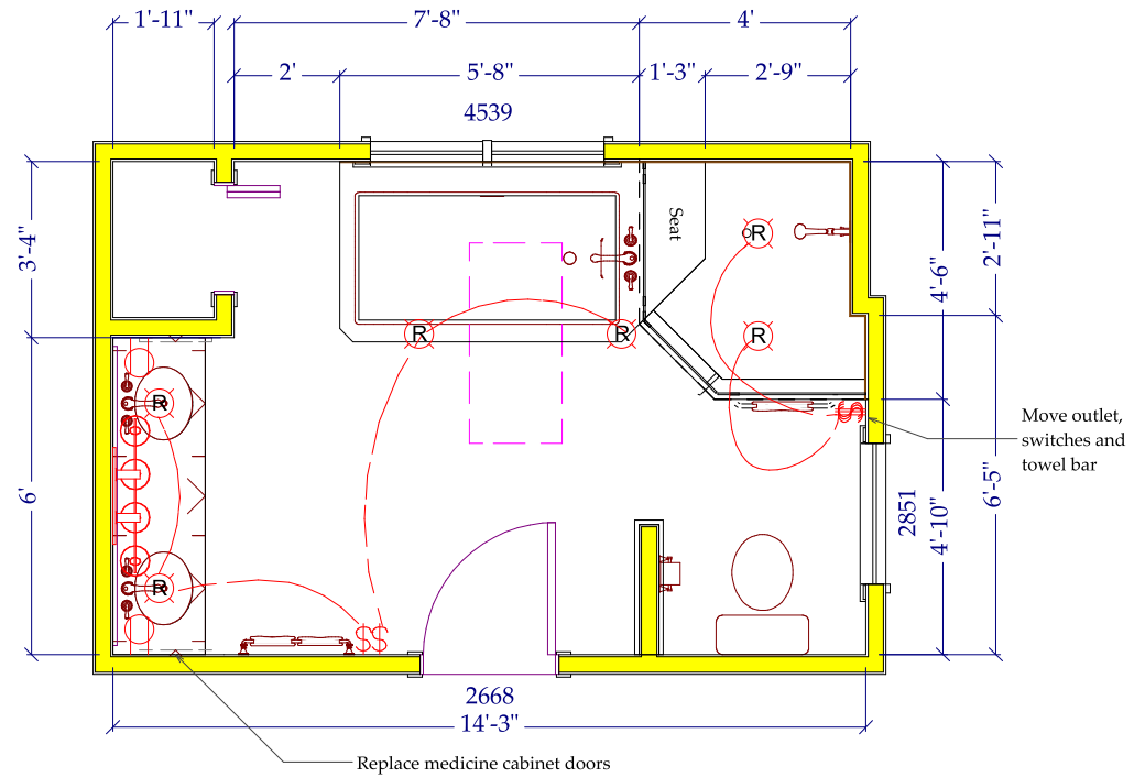
RENOVATED BATH LAYOUT
