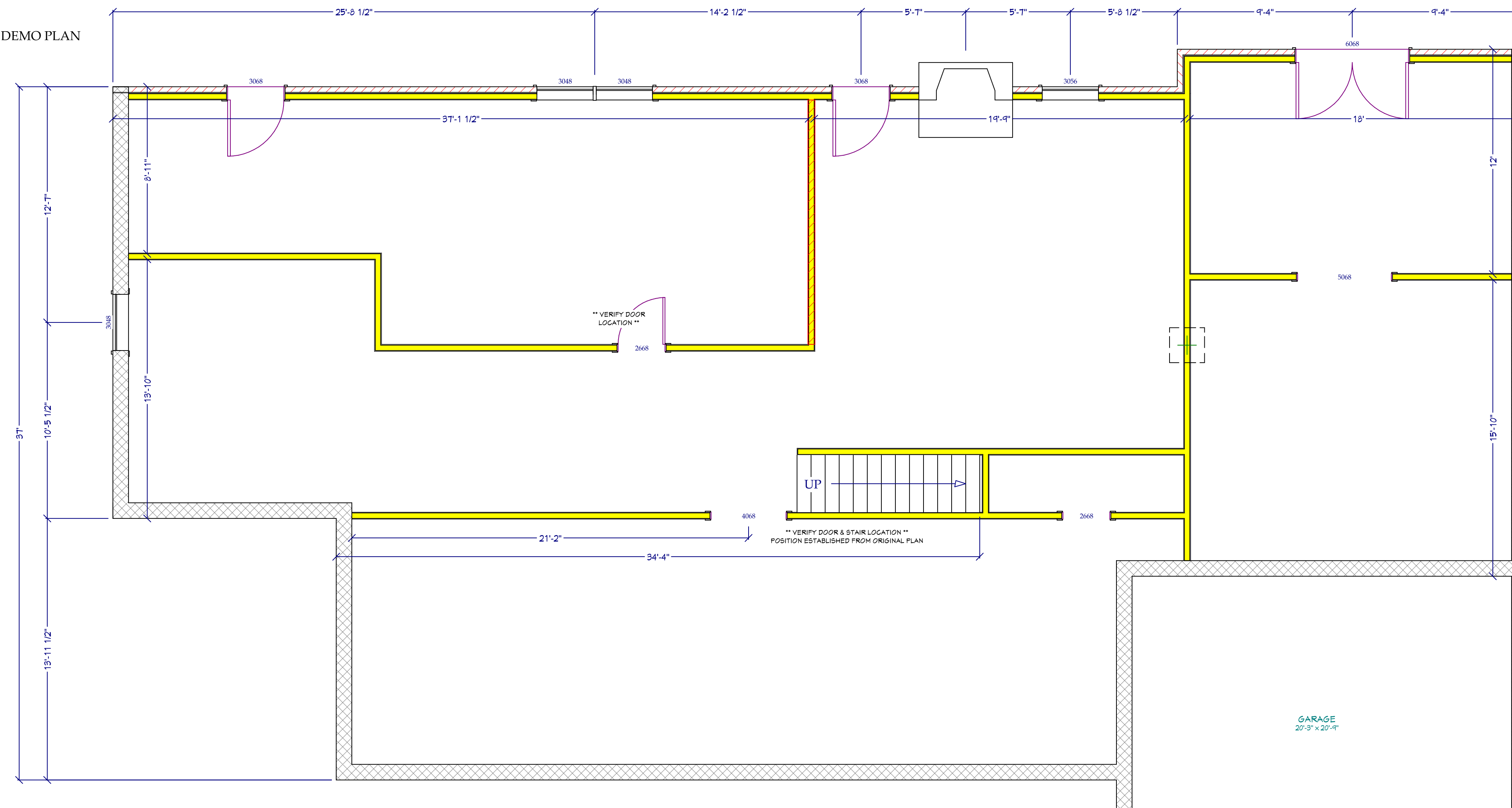
RENOVATED PLAN
