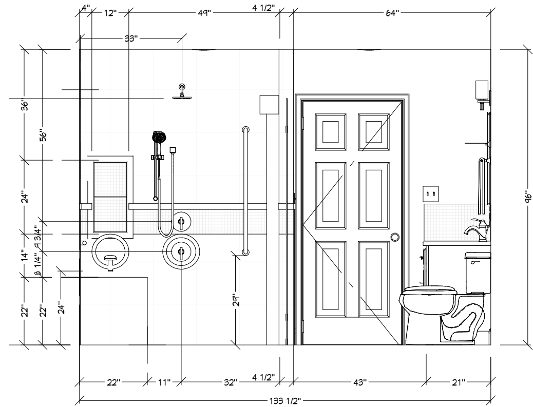
SHOWER RIGHT WALL ELEVATION
