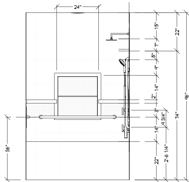
SHOWER BACK WALL ELEVATION
