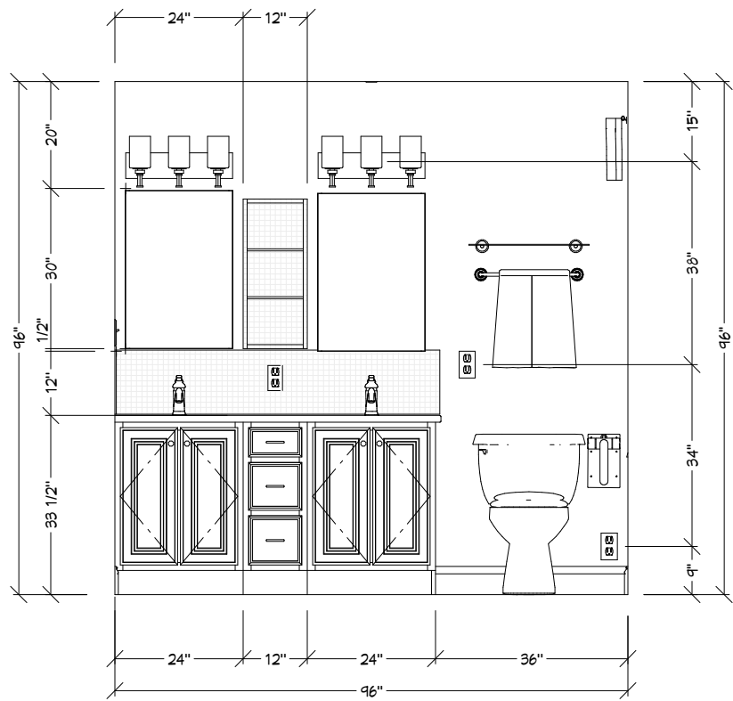
VANITY ELEVATION
