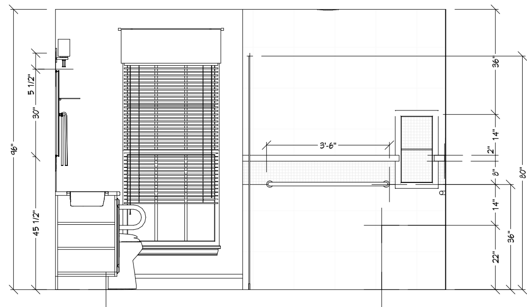
SHOWER LEFT WALL ELEVATION
